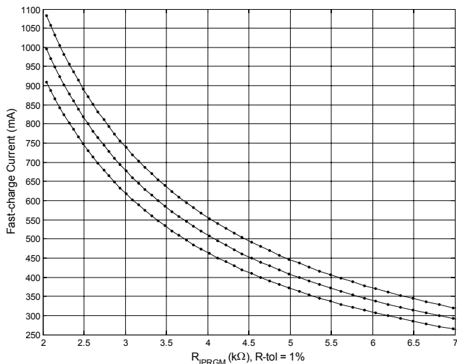
Figure 1a — Fast-charge Current Tolerance versus Programming Resistance, Low Resistance Range
