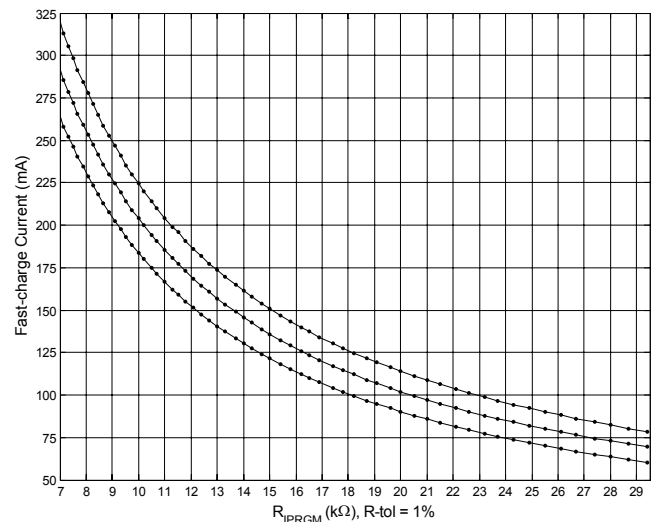
Figure 1b — Fast-charge Current Tolerance versus Programming Resistance, High Resistance Range
